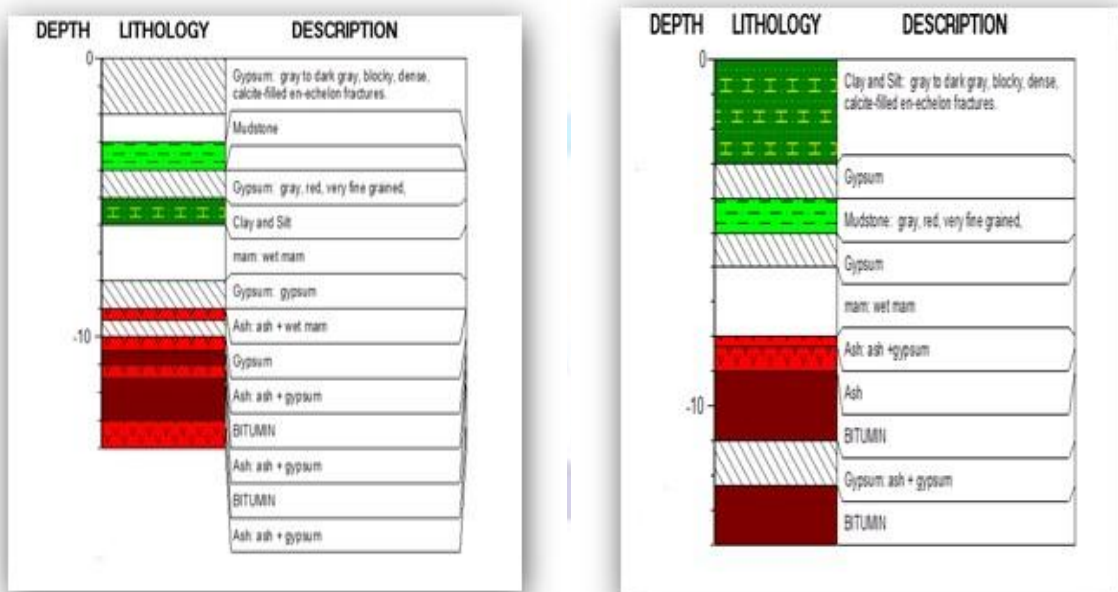
Figure7. Boreholes BH3 and BH4
