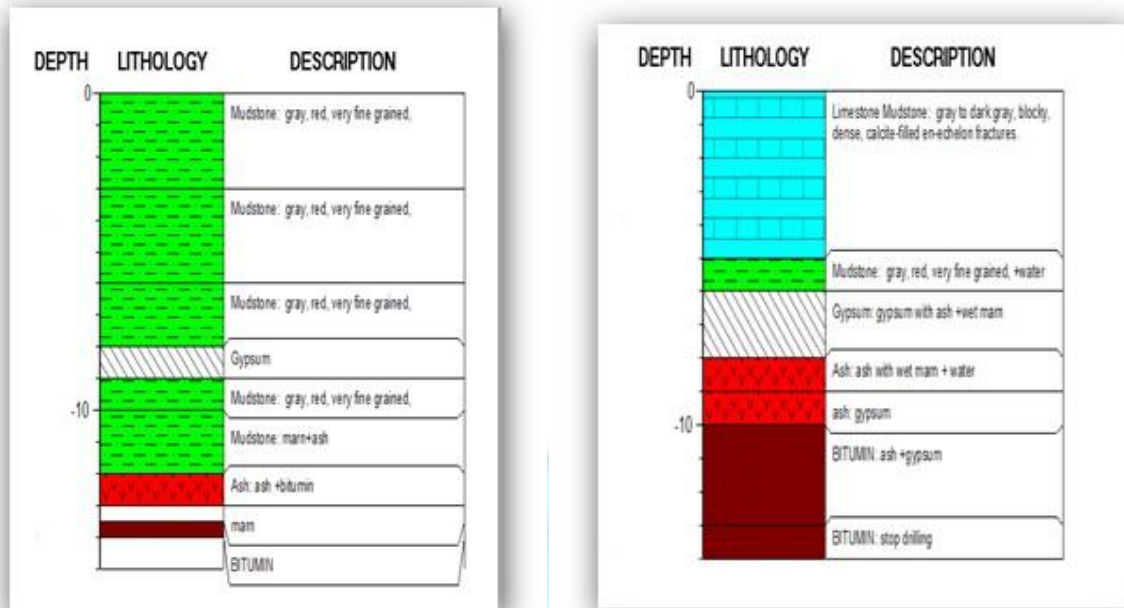
Figure6. Boreholes BH1 and BH2
