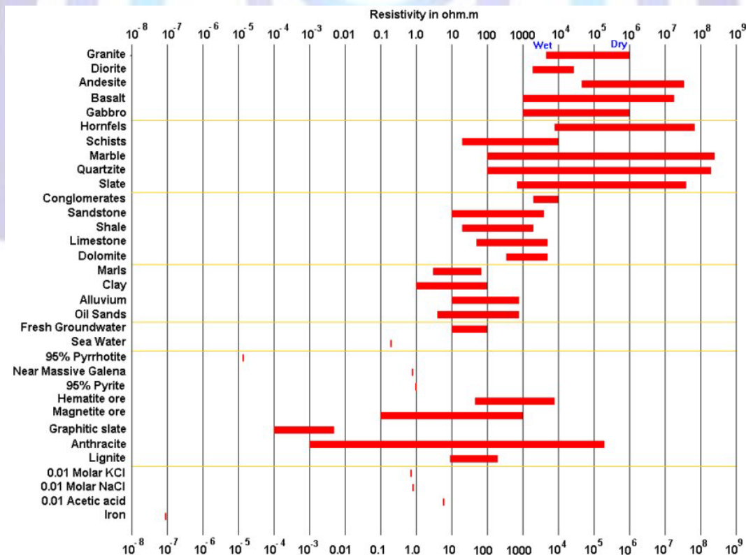
Figure1.Ground resistivity material
