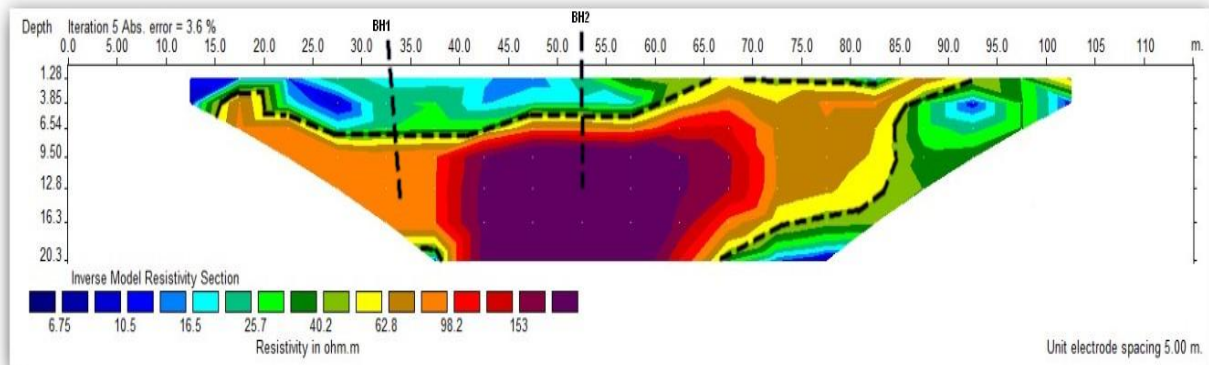
Figure4. Electrical resistivity pseudo-section profiles (1)
