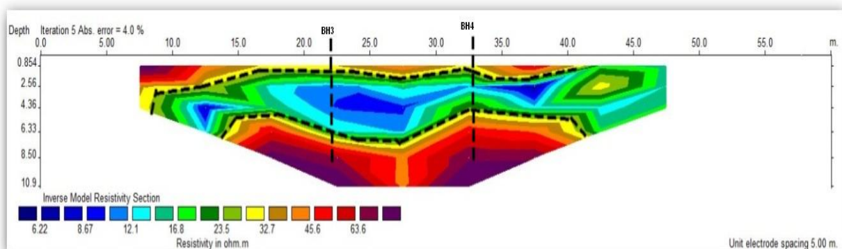
Figure5. Electrical resistivity pseudo-section profiles (2)
