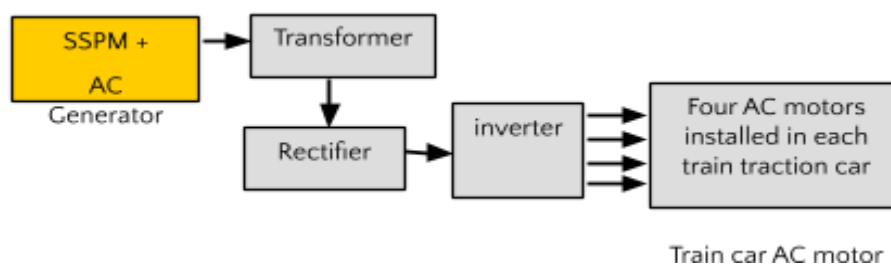
Figure 15. Illustration of a simplified architecture for a self-sustaining power supply system based on a SSPM to assist an electric traction system (ETS) that can be installed in a train traction car.
