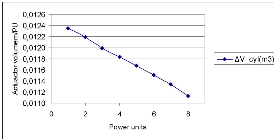
Figure8. illustration of the volume ( m^3 ) assigned to each PGT-based turbine
