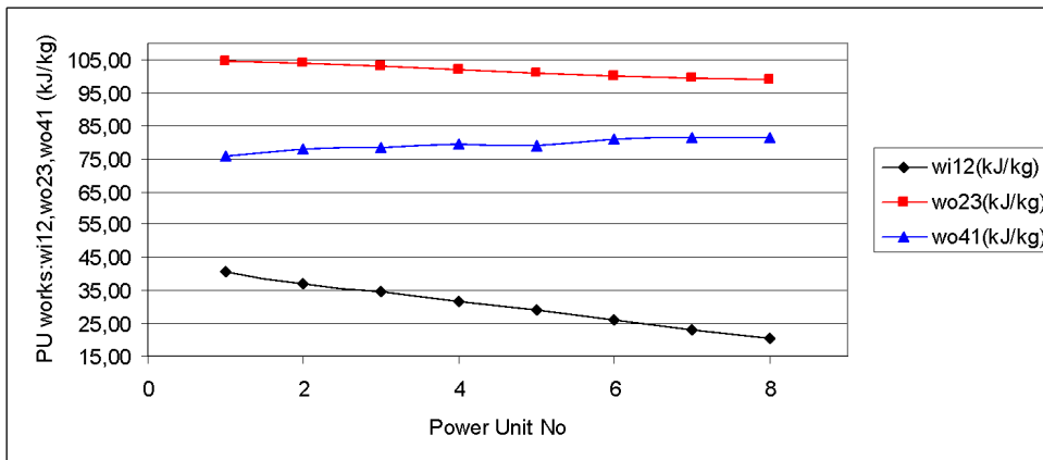
Figure 5. illustration of the input feed pump work, output expansion and output contraction works for the eight cascaded PUs
