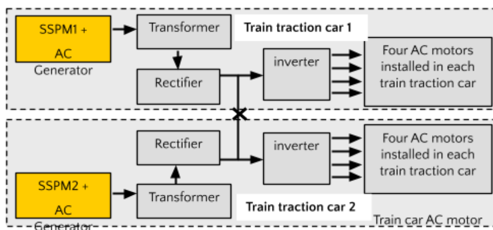
Figure 16. Illustration of a simplified architecture for a self-sustaining power supply system based on two independent SSPMs to assist an electric traction system (ETS) that can be installed in TWO train traction cars.
