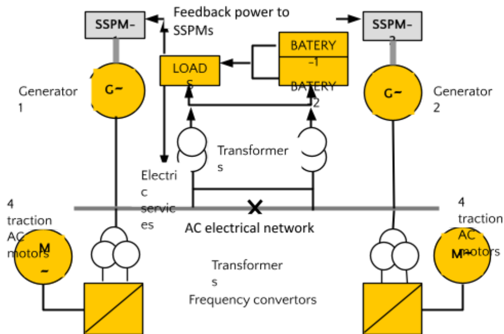
Figure 17. Illustration of a simplified architecture of a self-sustaining energy-assisted ETS adapted to feed two train traction cars.
