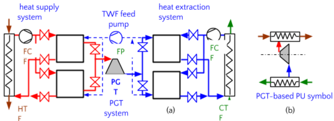
Figure 1. Illustration of the PGT based on the patent application number P202000032 and publication number ES2851381, [16], [20]. Figure 1(a) depicts the main subsystems including the heat supply system, the heat extraction system, the TWF feeding system and the PGT machine. Figure 1 (b) illustrates the symbol used to represent the PGT-based PU depicted in Figure 1(a).
