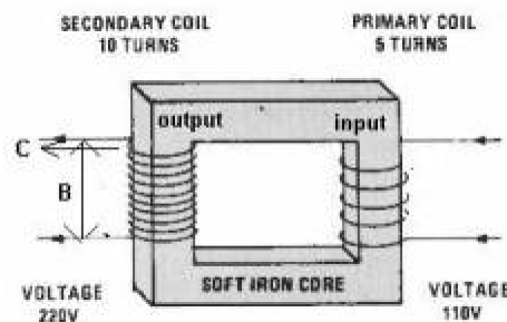
Figure 3: Magnetic frame serves as electrical generator.
