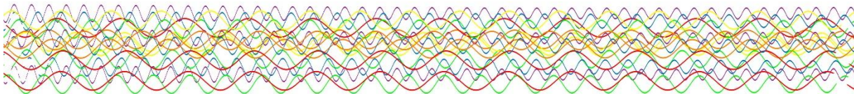
Fig. 6 : composition of a light beam observed along its side.
