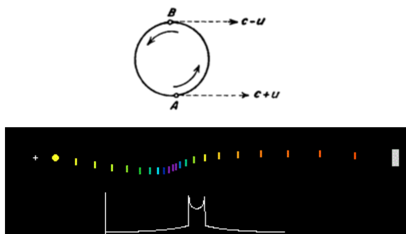
Fig. 8: De Sitter Spectroscopic Binaries experiment
