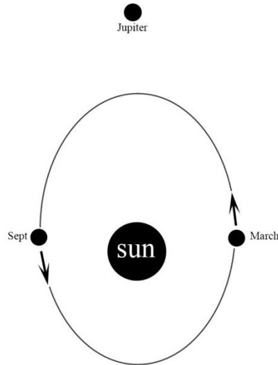
Fig.9: Earth's orbital ellipses relatively to Jupiter
