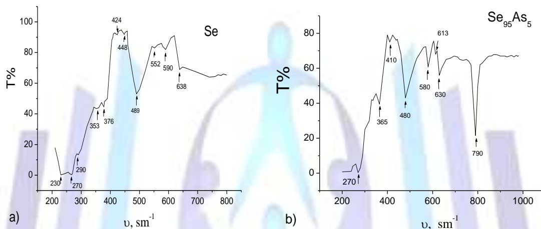
Fig.1. Spectrums of the infrared transmission of the amorphous selenium (a) and of \text{Se}_{95}\text{As}_5 system (b).
