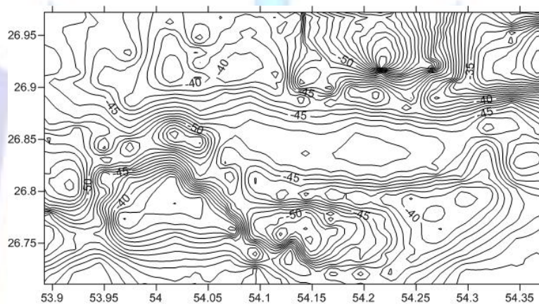
Figure (5): Contour map of complete bouguer anomaly with density (2.7)g/cm^3 and level line differences of 1 (m gal)
