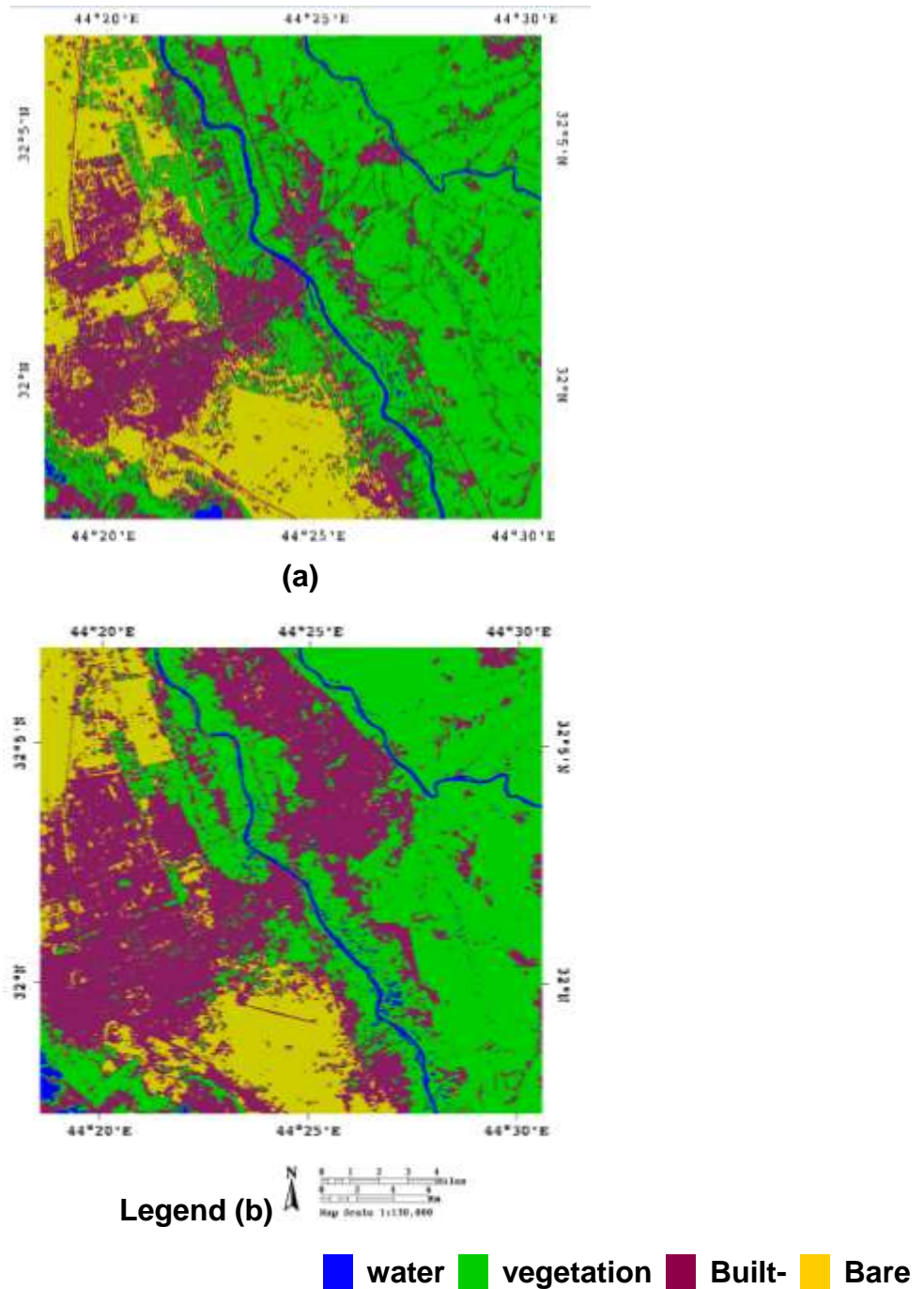
Figure 2: Results of Supervised classification for the study area(a) 1990, (b) 2009.
