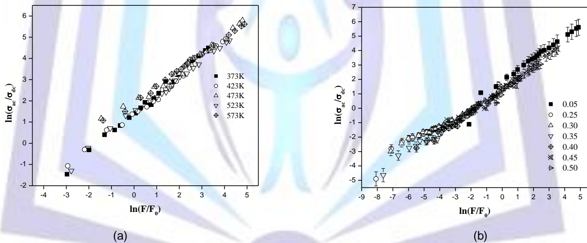
Fig 8: (a) The ac conductivity master curves for the BPCL1 glasses for different temperatures. (b) The ac conductivity master curves of all the BPCL glasses at 573K.
