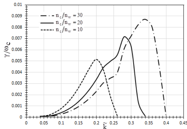
Fig 6. Variation of Growth Rate and Real Frequency with respect to \tilde{k} for various values of n_c/n_w at T_{\perp}/T_{\parallel} = 1.25 , n_o = 4 \times 10^4 \text{ m}^{-3} and other fixed plasma parameters.
