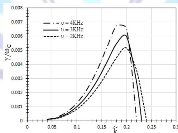
Fig 2. Variation of Growth Rate and Real Frequency with respect to \tilde{k} for various values of AC frequency \nu , at T_{\perp}/T_{\parallel} = 1.25 , n_o=4 \times 10^4 \text{ m}^{-3} and other fixed plasma parameters.
