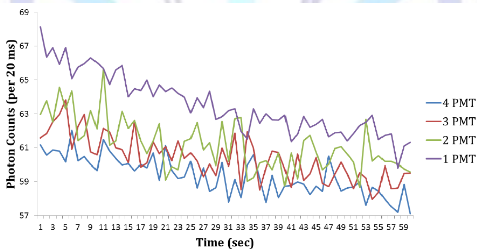
Figure 3. Averaged photon counts per 20 ms beginning 5 s after the offset of the LED during the subsequent 60 s from the reference photomultiplier unit when only the unit or 1, 2, 3 additional units were measuring photon counts simultaneously.
