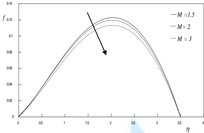
Fig.3 Effect of M on the primary flow velocity profiles f' with Gr = 0.1 , n=1.2 , s = 0.19 , \theta_x = 0.4 and m = 1
