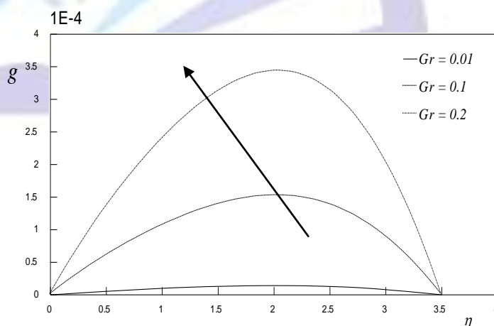
Fig.2. Effect of Gr on the secondary flow velocity profiles g with M = 0.1 , n = 1.2 , s = 0.19 , \theta_r = 0.4 and m = 1
