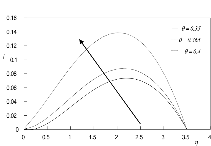
Fig.9 Effect of \theta_x on the primary flow velocity profiles f' with Gr = 0.1 , n=1.2 , M= 0.1 , s = 0.19 and m = 1
