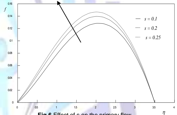
Fig.6 Effect of s on the primary flow velocity profiles f' with Gr = 0.1 , n=1.2 , M= 0.1 , \theta_x = 0.4 and m = 1
