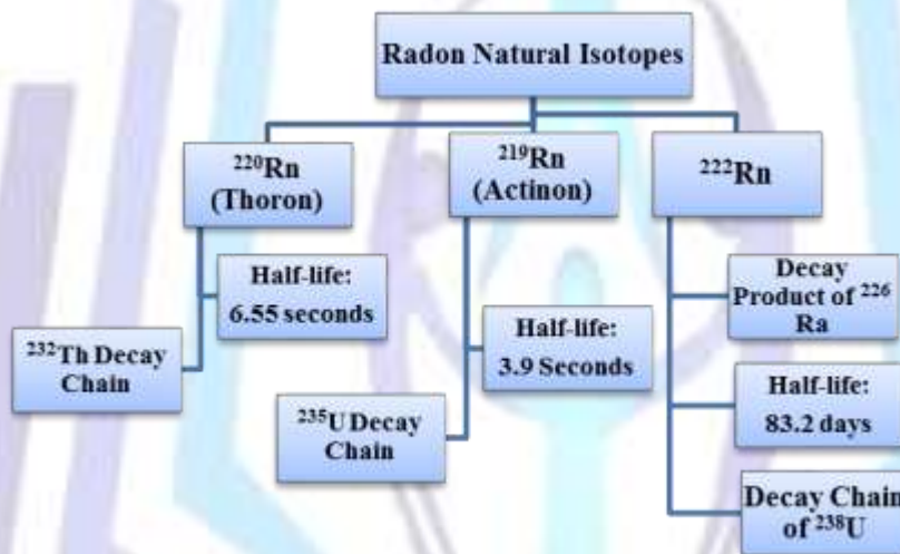
Figure 1: Different isotopes of Radon and its properties
