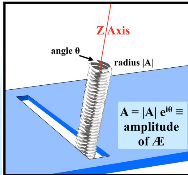
Fig 2: Sketch of an elementary ray \mathbb{R} of amplitude \mathbf{A} as it penetrates slit A
