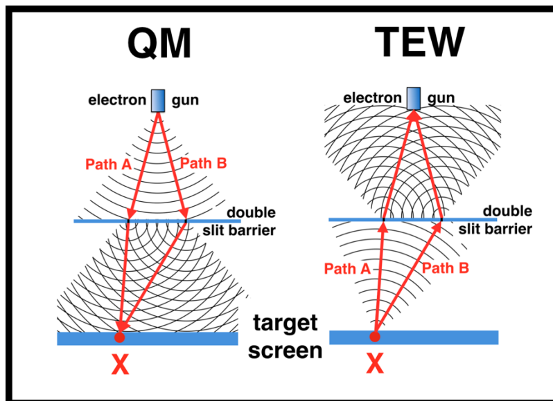
Fig 1: Comparing a QM picture to a TEW picture of a double slit experiment.
