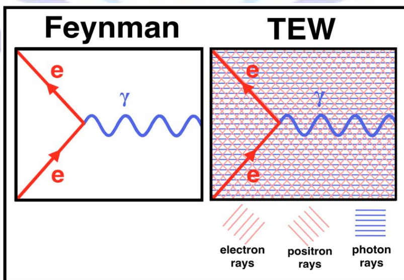
Fig 4. Comparing a Feynman and TEW view of the same particle annihilation and photon
