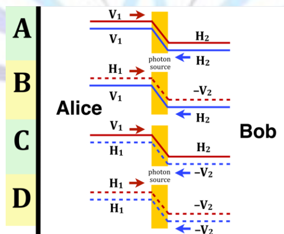
Fig 3 The four eigenstates (A, B, C & D) of the bi-ray (\hat{\mathbb{R}}_R \hat{\mathbb{U}} \hat{\mathbb{R}}_L) .
