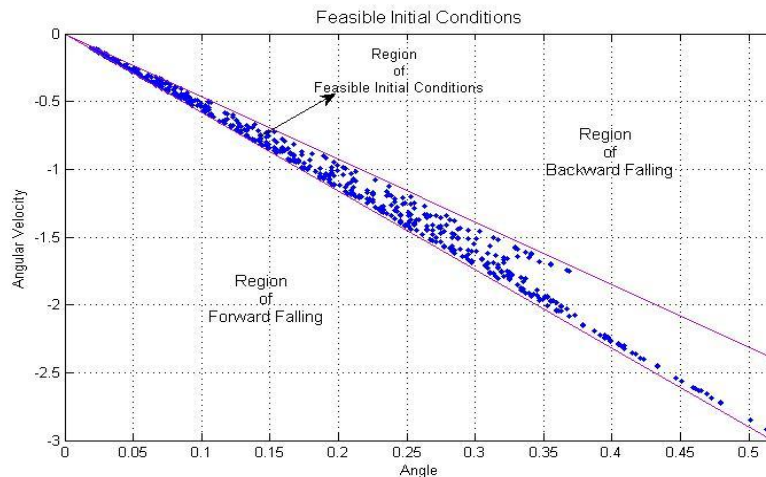
Fig 4: Feasible Initial conditions (\theta, \dot{\theta}) for the passive dynamic biped robot with respect to stance leg angle \theta and stance leg angular velocity \dot{\theta} jointly with region of forward falling and backward following at a ramp slope of \alpha = 0.0349 rad. (2°deg).
