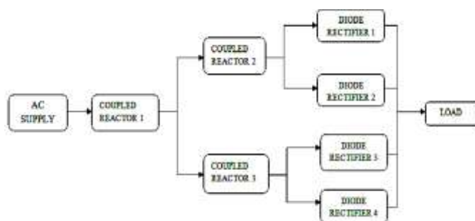
Fig.1. Block Diagram Of 24 Pulse Diode Rectifier
