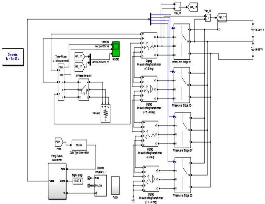
Fig. 4 Simulation block for 48 Pulse Diode Rectifier
