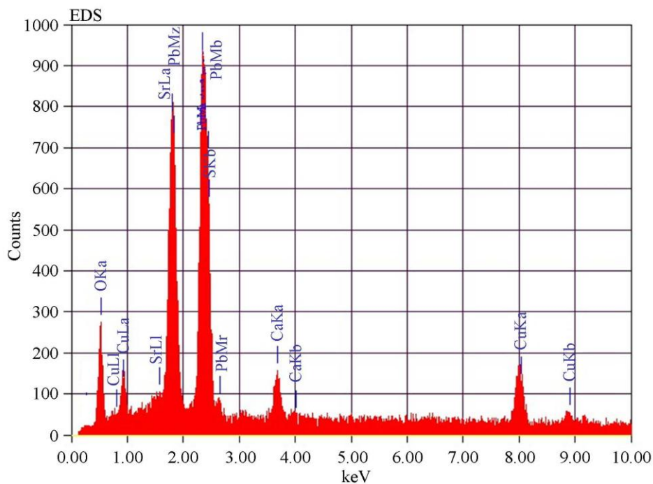
Figure 4. EDX of PbSrCaCuO
