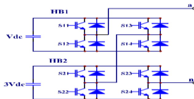
Fig1.Trinary Source MLI
