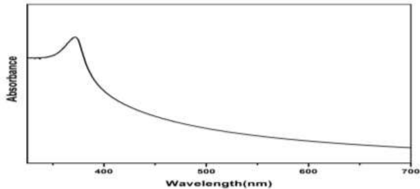
Fig. 3. UV-Vis spectroscopy of green synthesized ZnO nanoparticles.
