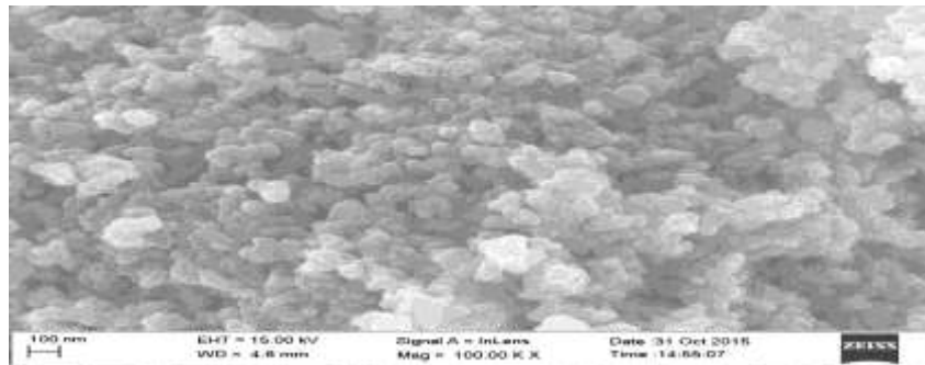
Fig. 2. FESEM image of green synthesized ZnO nanoparticles.
