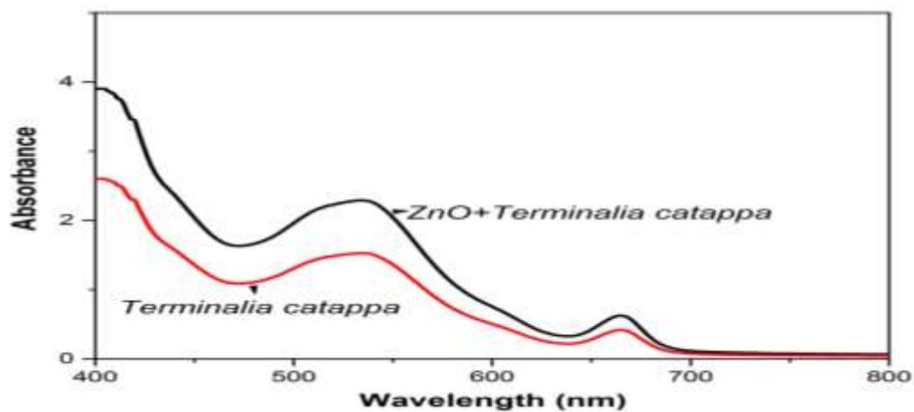
Fig. 4. Absorbance spectra of fruit extracts of Terminalia catappa and Terminalia catappa sensitized ZnO photo anode.
