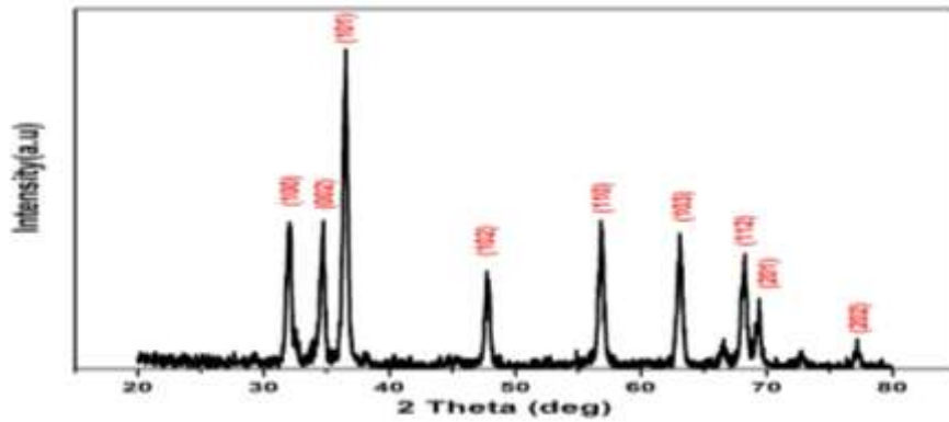
Fig. 1. XRD pattern of green synthesized ZnO nanoparticles.
