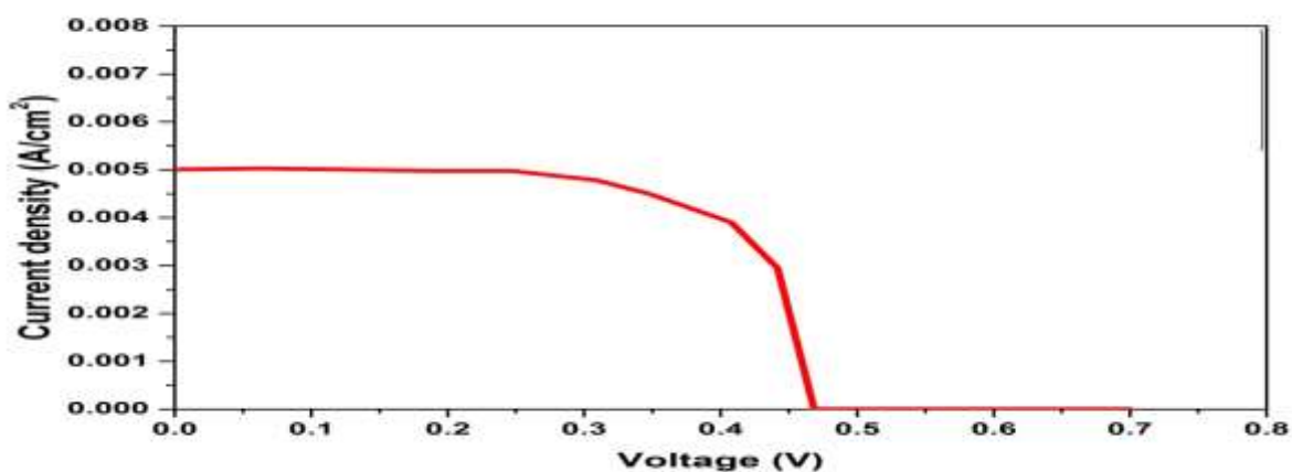
Fig 5 J-V characteristics of Terminalia catappa fruit extract sensitized solar cell.
