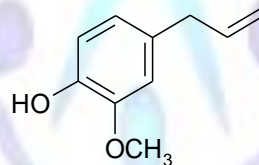
Fig. 3. Chemical structure of Eugenol
