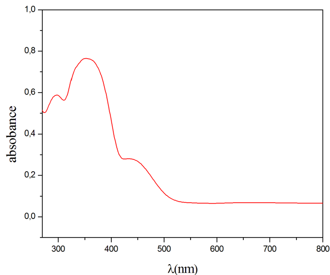
Figure 5. UV-Vis absorption spectrum of [\text{C}_9\text{H}_{14}\text{N}]_2\text{Cr}_2\text{O}_7
