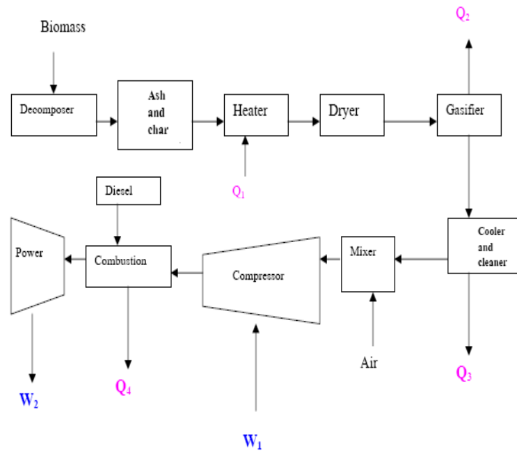
Figure 7 Advanced biomass power with diesel engine (Omer, 2006).
