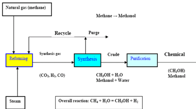
Figure 2 Schematic diagram shows methanol production (Omer, 2006).
