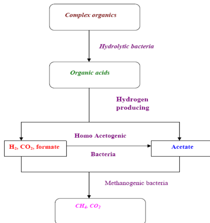
Figure 3 Biogas production process (Omer, 2003).
