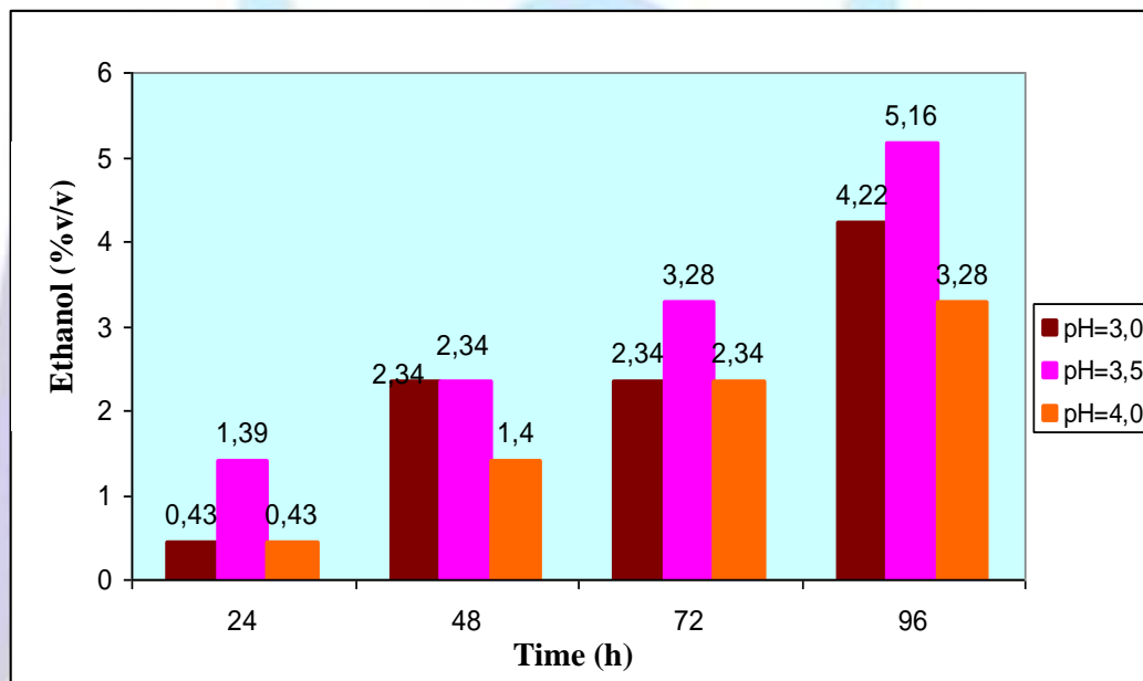
Figure 3. Effect of initial pH to ethanol formation in fermentation
