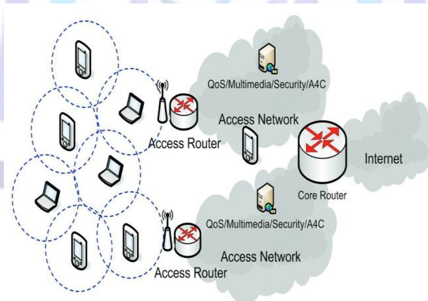
Fig3: Architecuture of MANET
