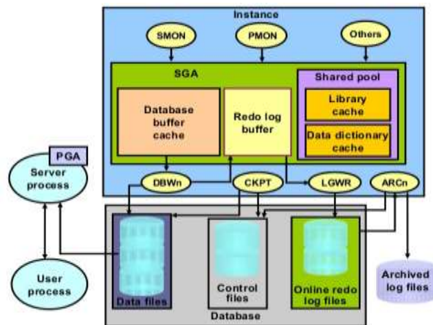
Fig 1: Database Architecture
