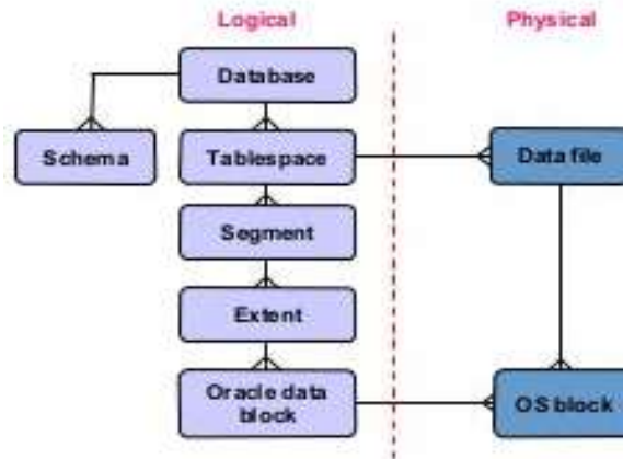
Fig 2: Memory Structure
