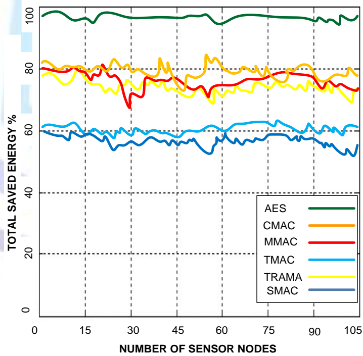
Fig 5. Total Energy saving for number of sensors
