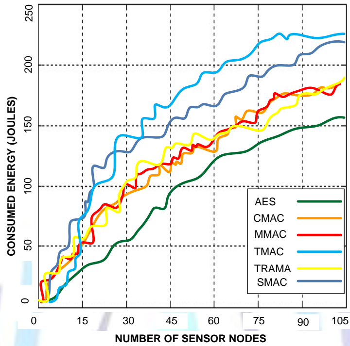
Fig 4: Energy consumption at different number of sensors
