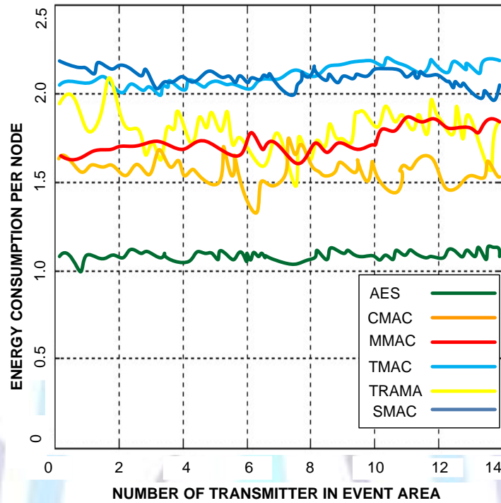
Fig 6: Consumption of energy at different transmitters
