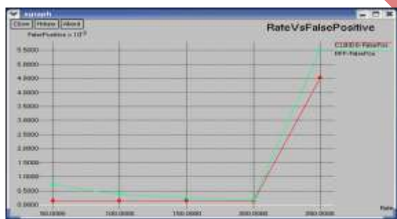
Figure shows the false positive rate of our cross-layer technique and RFF. From the figure, one can observe that our cross-layer scheme attains low false positive rate, when compared with RFF scheme, since it accurately detects the intrusion.
