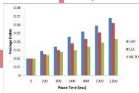
Figure 4. Average delay with pause time
