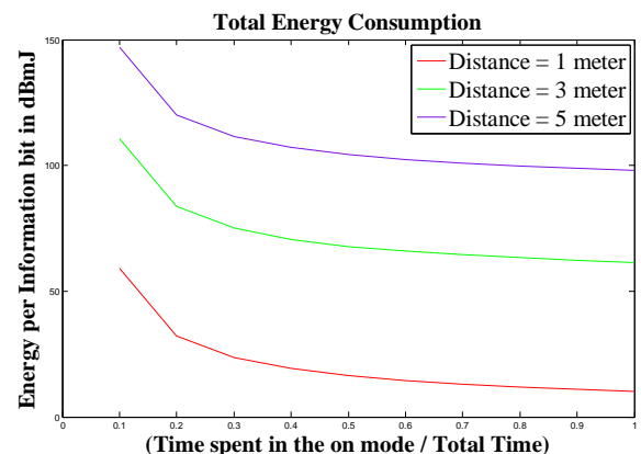
Figure 1: Total Energy Consumption per bit versus Time Spent in the On mode / Total Time for different distances at a packet size of 2000 bits.
