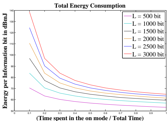
Figure 2: Total Energy Consumption per bit versus Time spent in the On mode / Total Time for different packet sizes at a distance of 3 meters.
