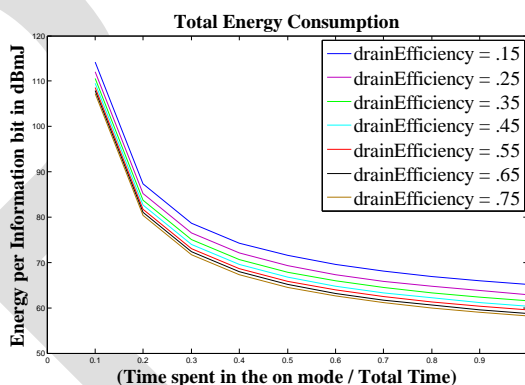
Figure 5: Total Energy Consumption per bit versus Time Spent in the On mode / Total Time for different drain Efficiency at a distance of 3 meters.
