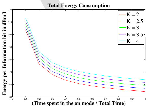
Figure 3: Total Energy Consumption per bit versus Time Spent in the On mode / Total Time for different path loss exponent (k) at a distance of 3 meters.
