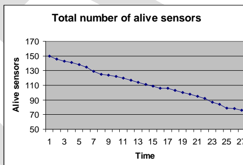
Figure 29: Total number of alive sensors over the life cycle
