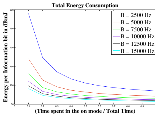
Figure 4: Total Energy Consumption per bit versus Time Spent in the On mode / Total Time for different bandwidth at a distance of 3 meters.
