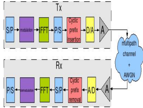
Fig.2. OFDM Transceiver Structure
