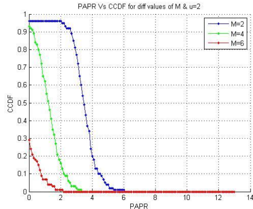
Figure 3 (PAPR vs CCDF for different value of M & u=2 )
