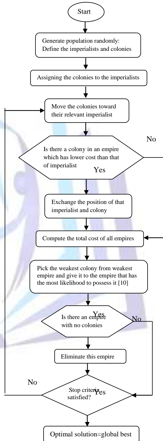
Figure 2. Flowchart of ICA algorithm
