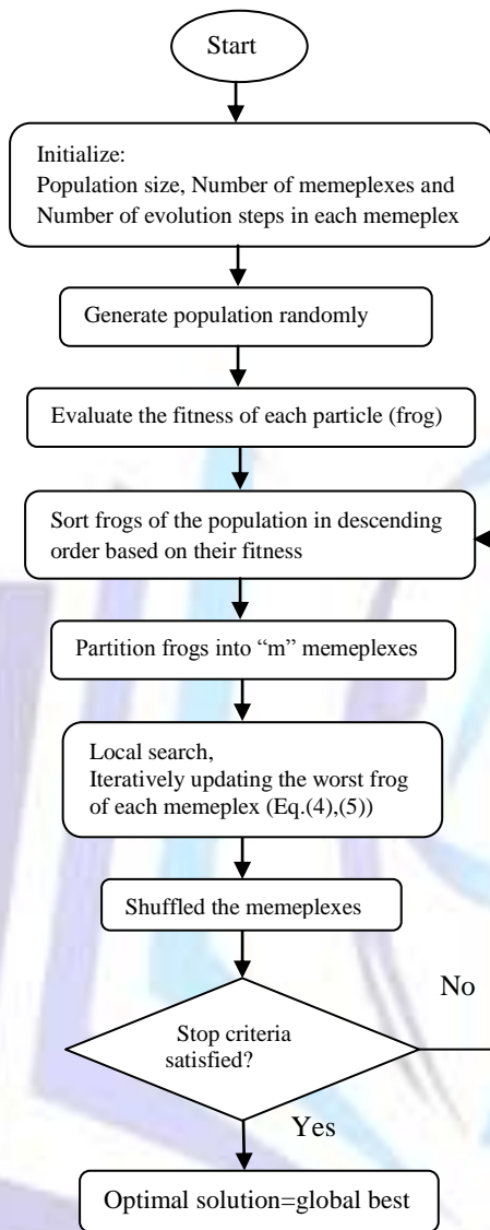
Figure 1. Flowchart of SFLA algorithm
