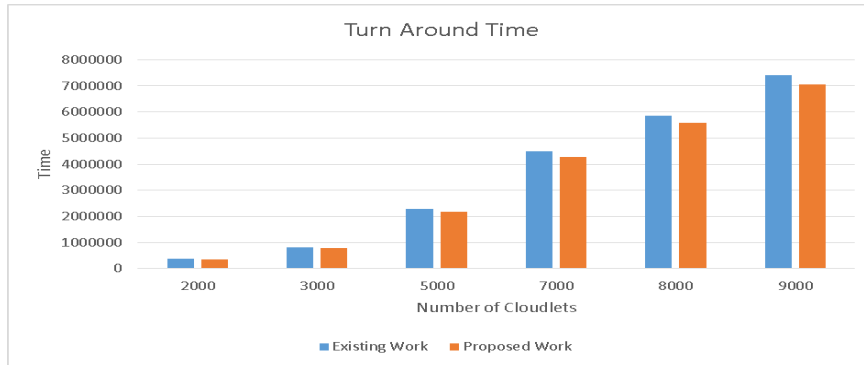
Figure 3. Turn Around Time
