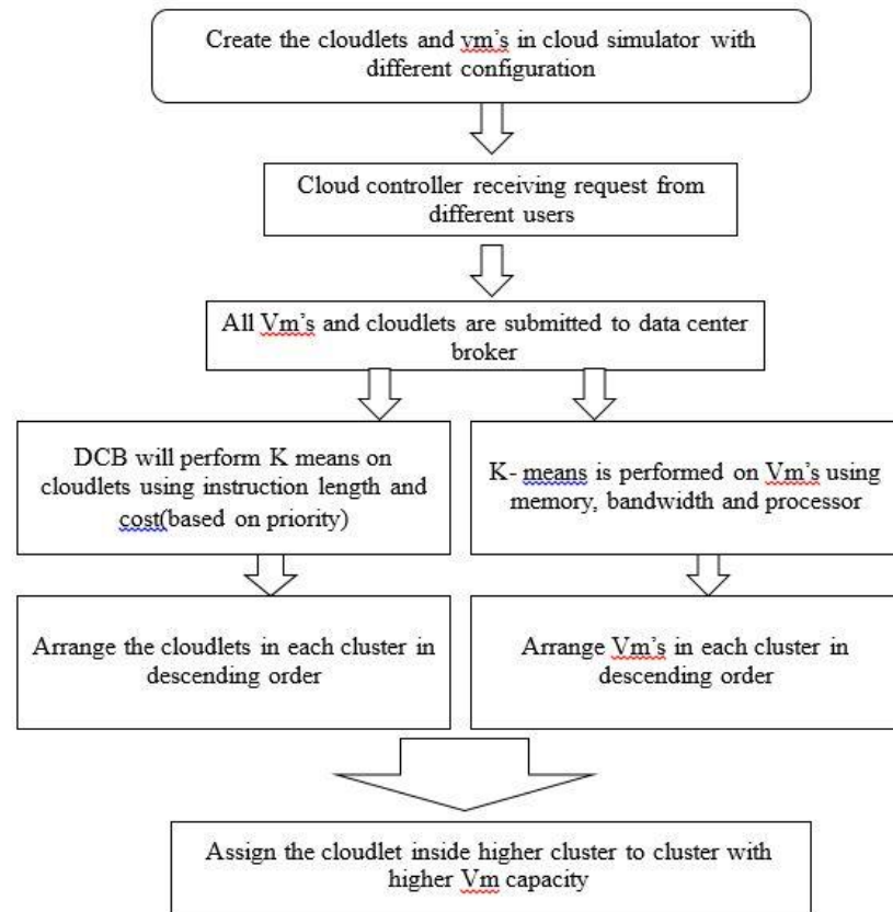
Figure 2. Flow Chart of the Proposed Work
