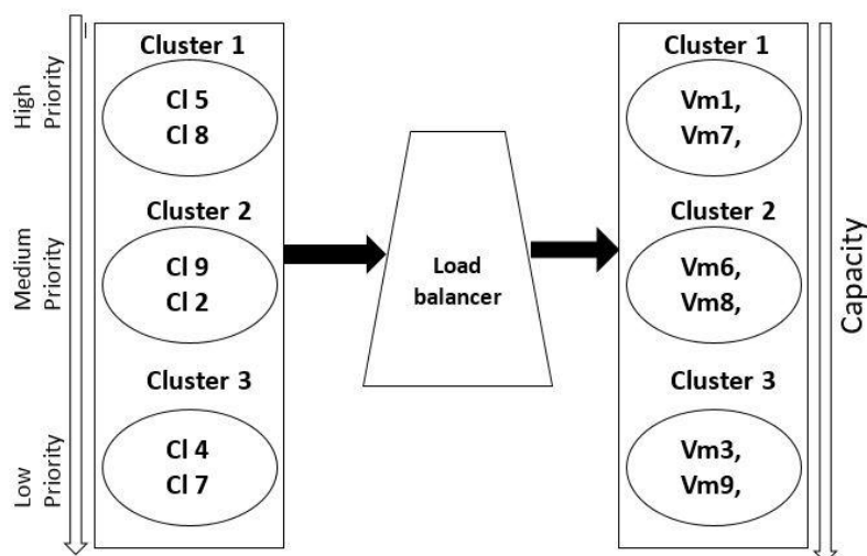
Figure 1. Proposed Load Balancing Model
